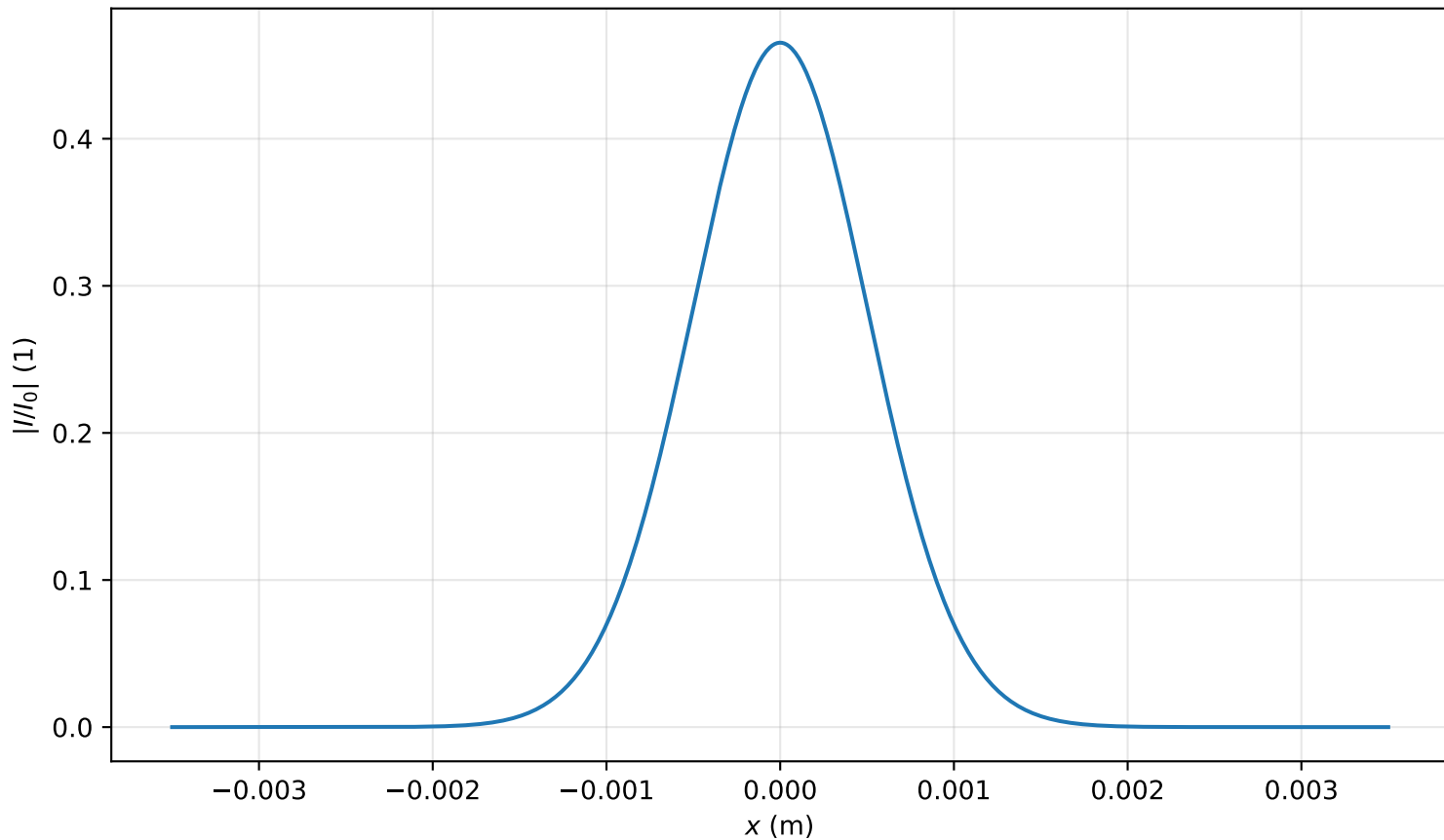
Intensity profile I(x, y = 0, z = 2.309m)/I_0 , P_{in}=0.1P_{cr} , artificial time
